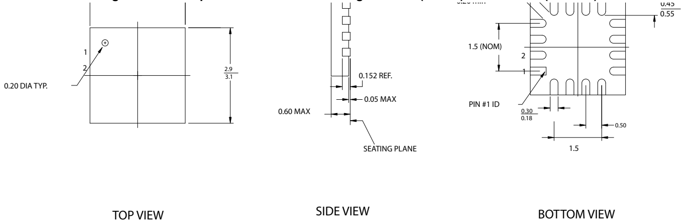
Figure 4. 16L Chip On Lead 3 X 3 mm Package Outline (SAWN) - 001-09116 - (Pb-Free)
