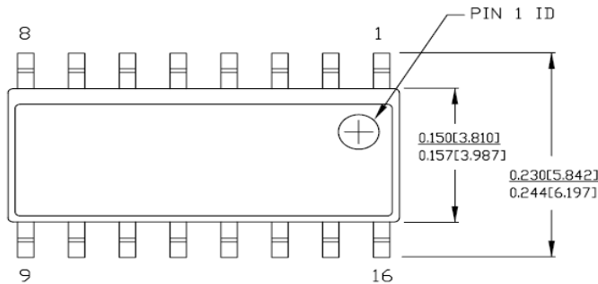
Figure 5. 16 - Pin (150-Mil) SOIC (51-85068)
